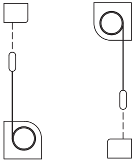
Vertical-Up Installation Vertical-Down Installation
